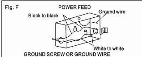
Wiring Connection in J-box for low voltage
