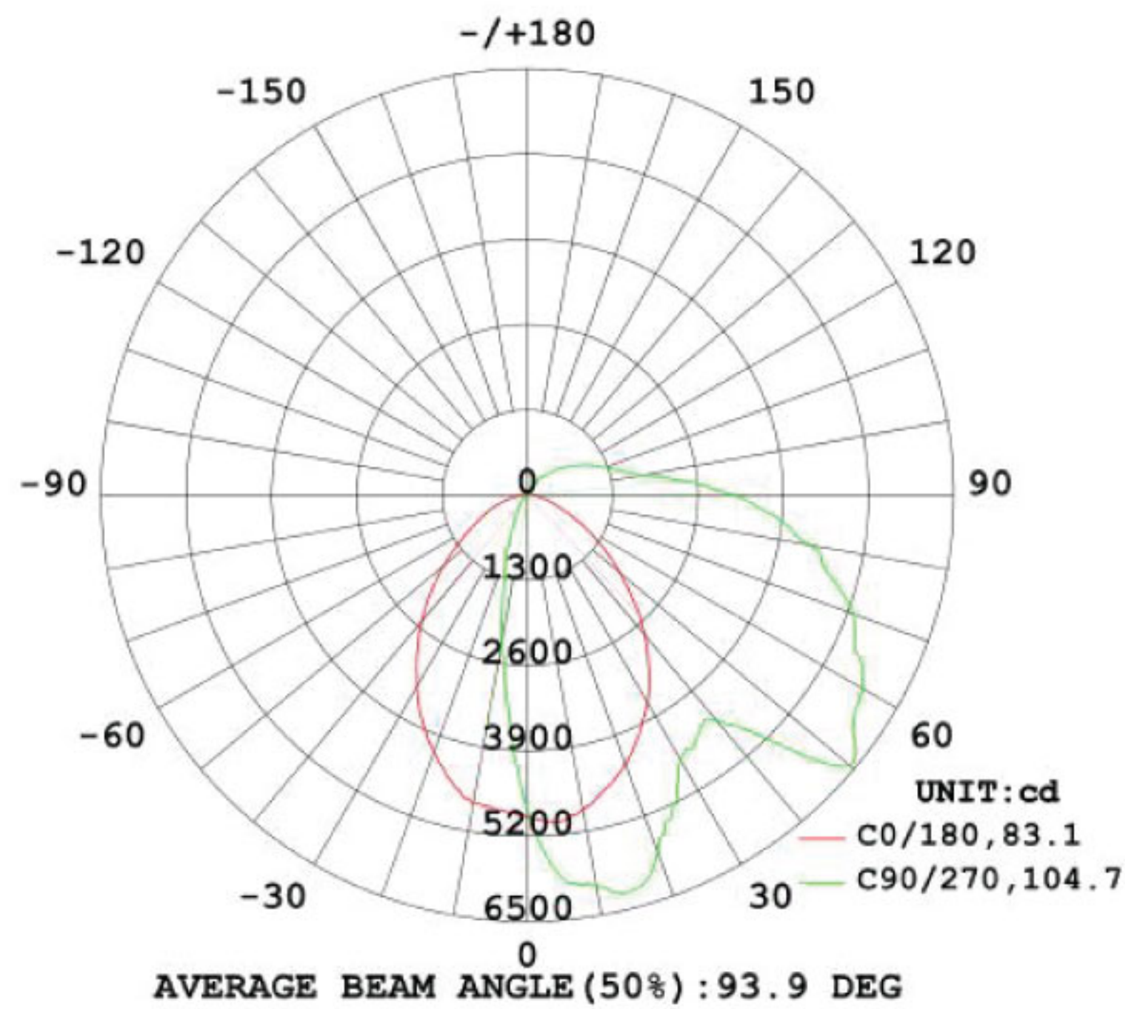
LUMINOUS INTENSITY DISTRIBUTION DIAGRAM
