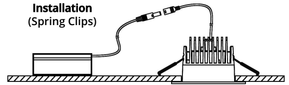
Installation (Spring Clips) Cutout: Ø 3-47/64" (95mm)
