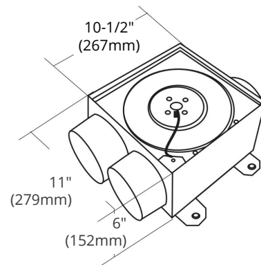
SDF200 Dimensions Diagram
